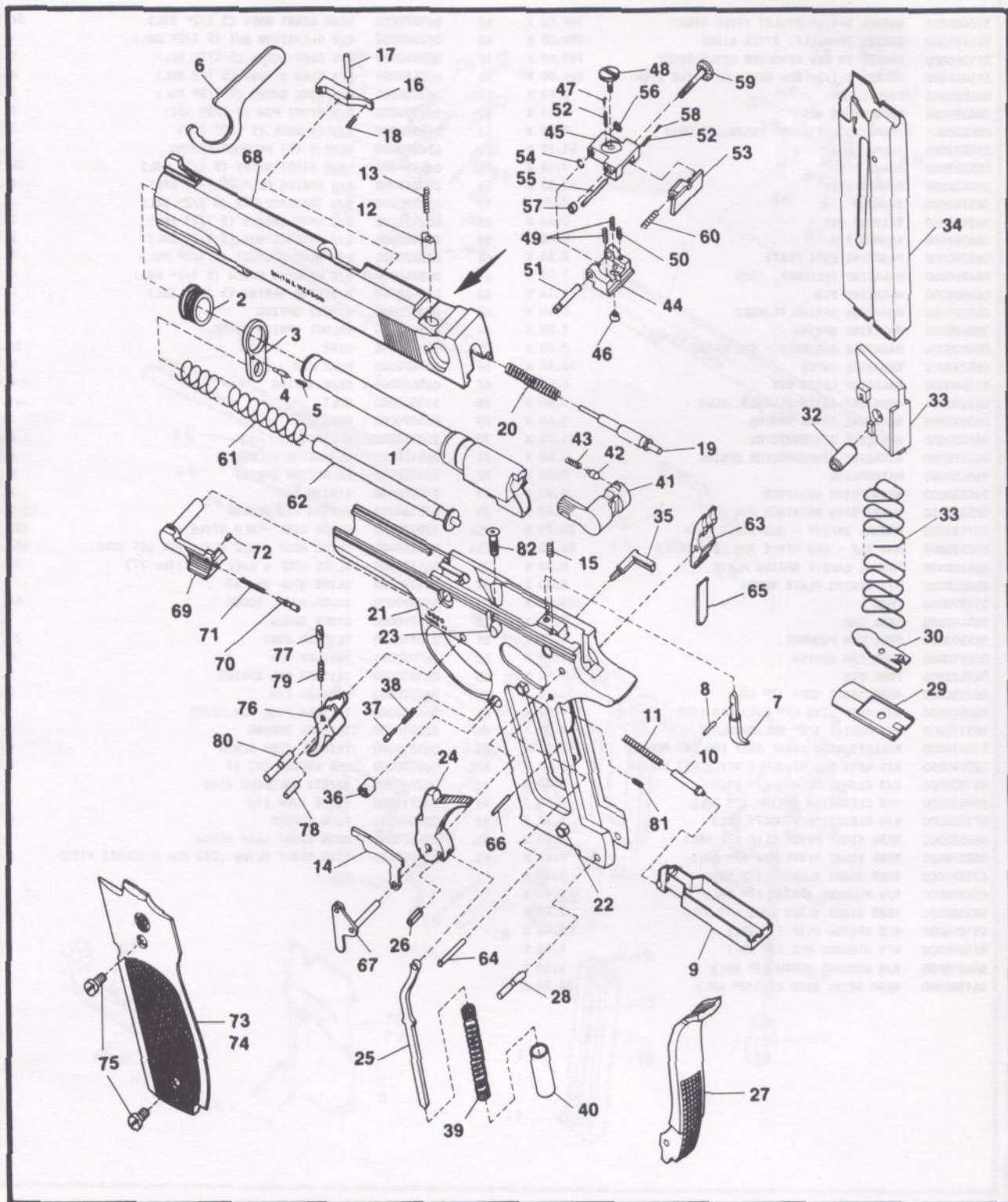
EXPLODED VIEW DIAGRAM.
