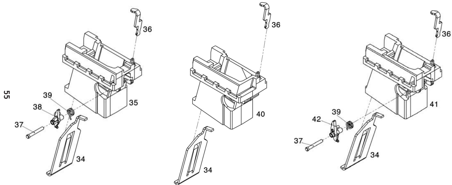
SR9®/SECURITY-9® ASSEMBLY (“SR9 S9” or “R9 R40”)
