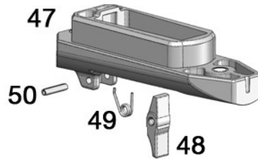
Mini-30 Magazine Well Assembly
