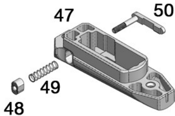
AR-15-Style Magazine Well Assembly
